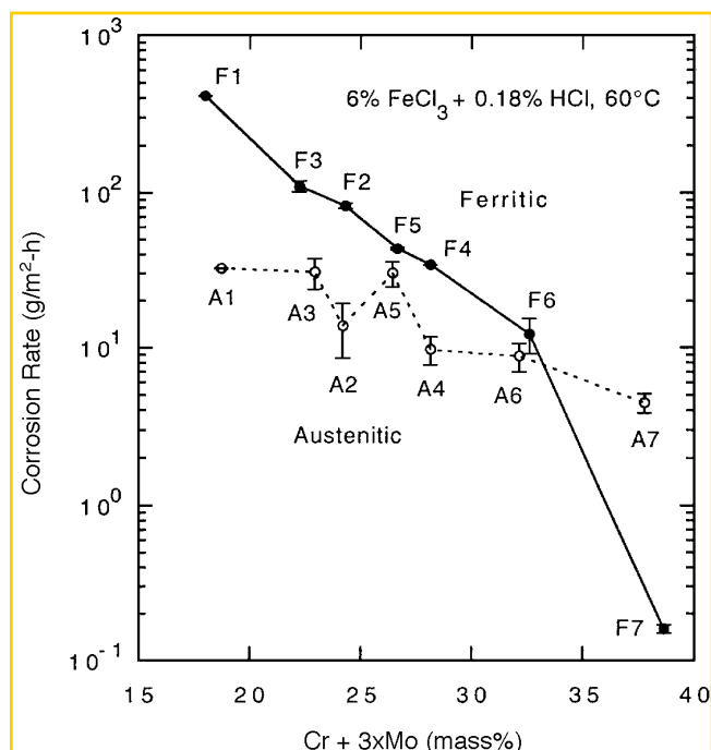
FIGURE 1. Pitting corrosion rate vs the Cr + 3xMo index for ferritic and austenitic SS exposed to 6% \text{FeCl}_3 + 0.18% HCl at 60°C.
